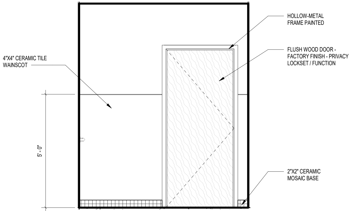
① TOILET - NORTH - AMENDED PERMIT 1/2" = 1'-0"
